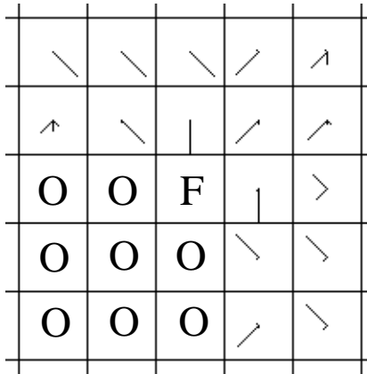
Figure 4. Example of predominant learned move directions in Woods1.
